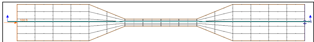
Figure 8 Observation arc through the constrained flume
